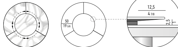
DETTAGLIO LAZY SUSAN | LAZY SUSAN DETAIL
