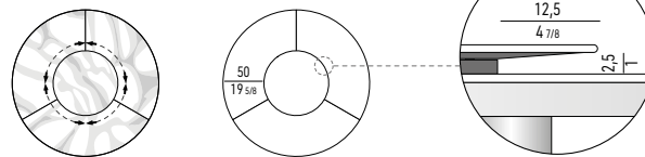
DETTAGLIO LAZY SUSAN | LAZY SUSAN DETAIL
