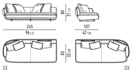
ELEMENTO TERMINALE CM 245 ELEMENT WITH 1 ARMREST CM 245
