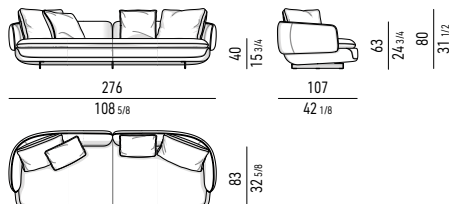
DIVANO CM 276 SOFA CM 276
