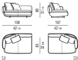
ELEMENTO TERMINALE CM 158 ELEMENT WITH 1 ARMREST CM 158
