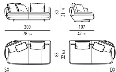
ELEMENTO TERMINALE CM 200 ELEMENT WITH 1 ARMREST CM 200
