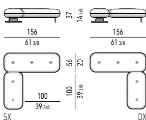
PANCA CM 156X156 BENCH CM 156X156
