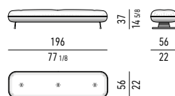
PANCA CM 196X56 BENCH CM 196X56
