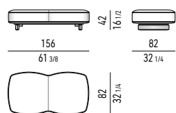
PANCA CM 156X82 BENCH CM 156X82
