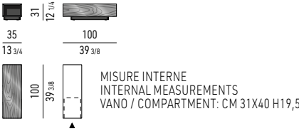
TAVOLINO CM 35X100 H31 CON 1 VANO INTERNO COFFEE TABLE CM 35X100 H31 WITH 1 INNER COMPARTMENT
