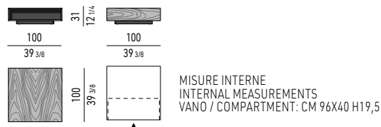
TAVOLINO CM 100X100 H31 CON 1 VANO INTERNO COFFEE TABLE CM 100X100 H31 WITH 1 INNER COMPARTMENT
