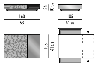
TAVOLINO CM 160X105 H26 COFFEE TABLE CM 160X105 H26
