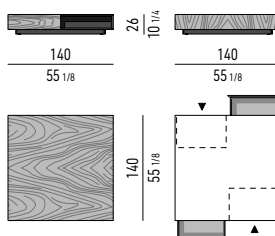
TAVOLINO CM 140X140 H26 COFFEE TABLE CM 140X140 H26
