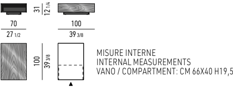
TAVOLINO CM 70X100 H31 CON 1 VANO INTERNO COFFEE TABLE CM 70X100 H31 WITH 1 INNER COMPARTMENT
