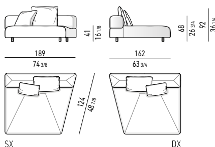
ANGLED COUCH CM 189X162 ANGLED COUCH CM 189X162
