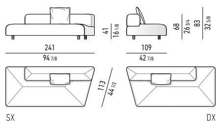
ANGLED ELEMENTO PENISOLA CM 241 - SCHIENALE CM 189 ANGLED OPEN-END ELEMENT CM 241 - BACKREST CM 189
