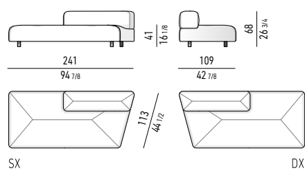
ANGLED ELEMENTO PENISOLA CM 241 - SCHIENALE CM 136 ANGLED OPEN-END ELEMENT CM 241 - BACKREST CM 136
