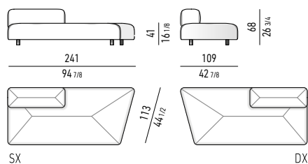
ANGLED ELEMENTO PENISOLA CM 241 - SCHIENALE CM 136 ANGLED OPEN-END ELEMENT CM 241 - BACKREST CM 136
